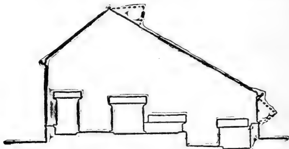
FIG. 107. FORCING HOUSE ( Section ).
